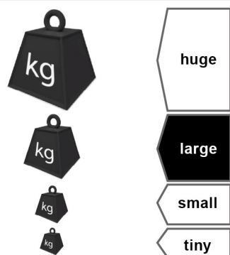
Chart 2 - How Big?
