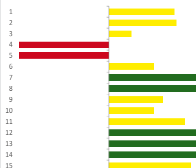
Spain KFSI-Assessment
